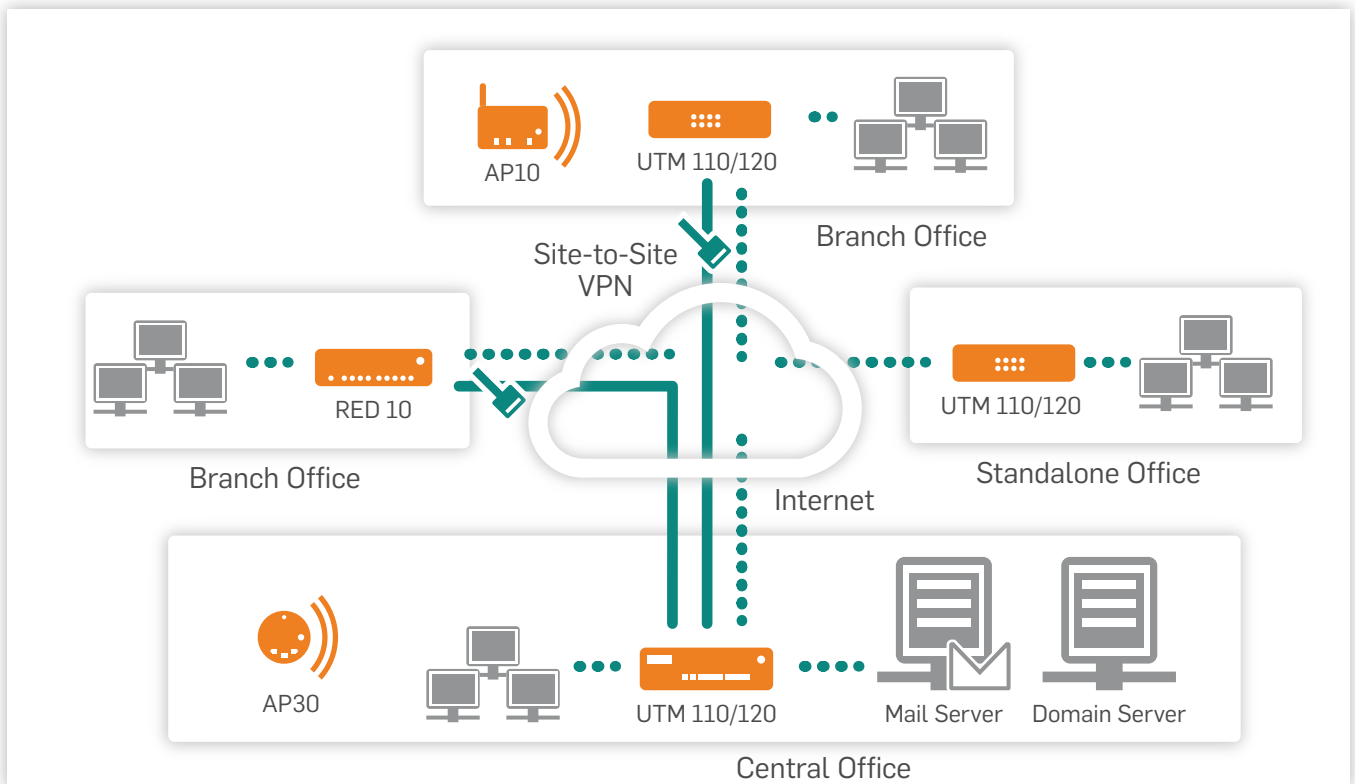
Deployment scenario of Sophos UTM 110/120
